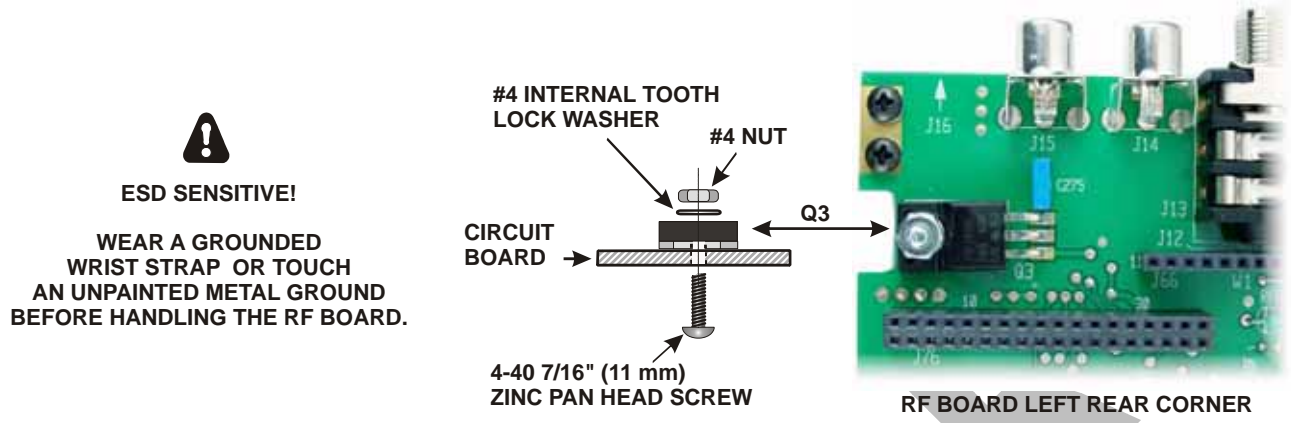
Figure 10. Installing Q3 Hardware on RF Board.
