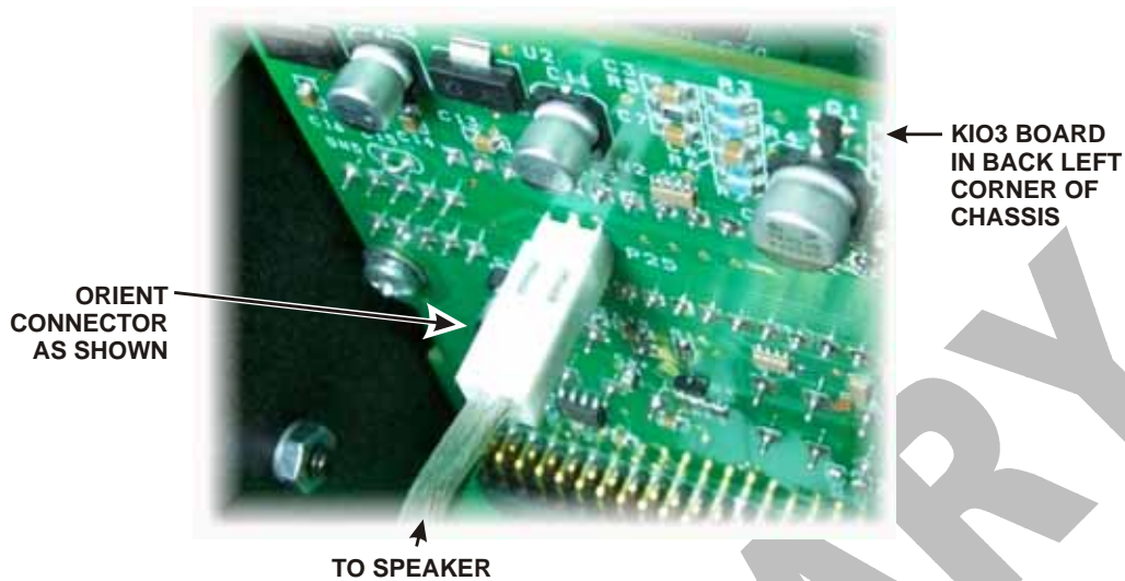
Figure 62. Connecting Speaker to KIO3 Board.
