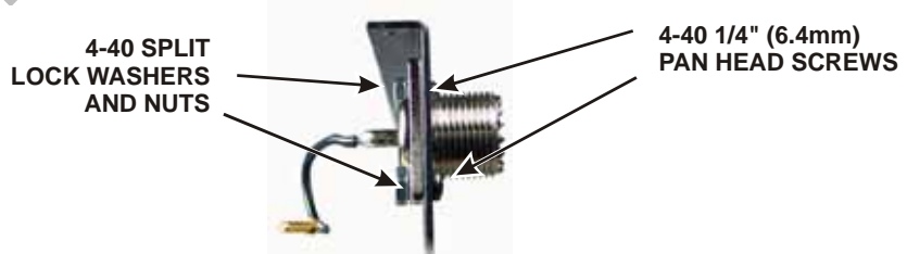
Figure 21. Mounting the ANT1 Connector.
