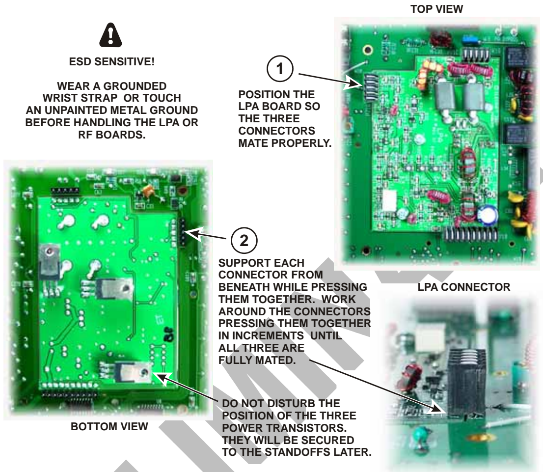
Figure 13. Installing the Low Power Amplifier (LPA).
