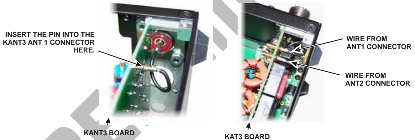
Figure 26. ANT Connections to KANT3 or KAT3 Boards.
