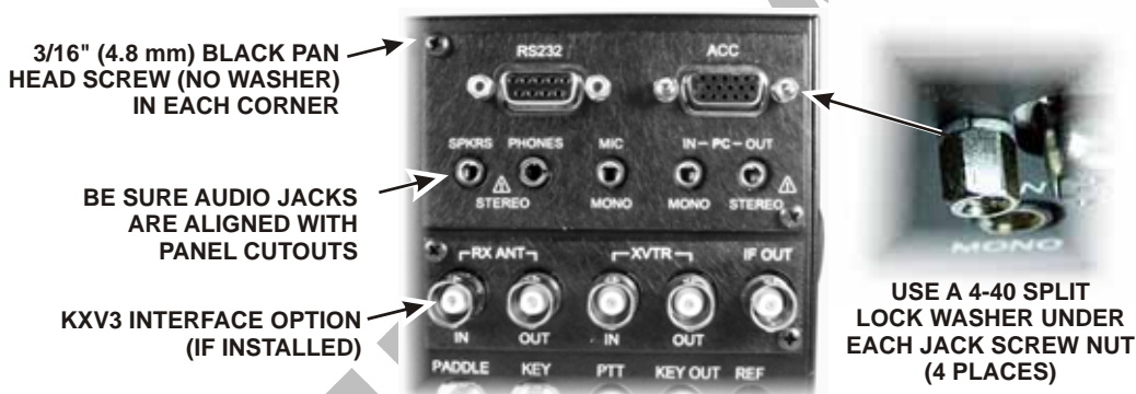
Figure 34. Mounting KIO3 Connector Panel.
